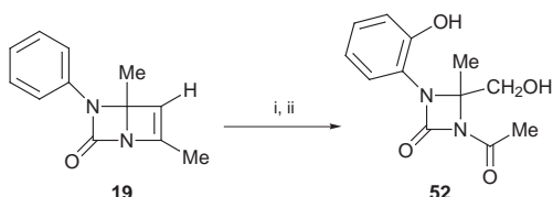
Scheme 10 Reagents and conditions: i, \text{O}_3 , \text{CH}_2\text{Cl}_2 – \text{MeOH} , -78^\circ\text{C} ; ii, \text{NaBH}_4 , 0^\circ\text{C} , 1 h, 40%
